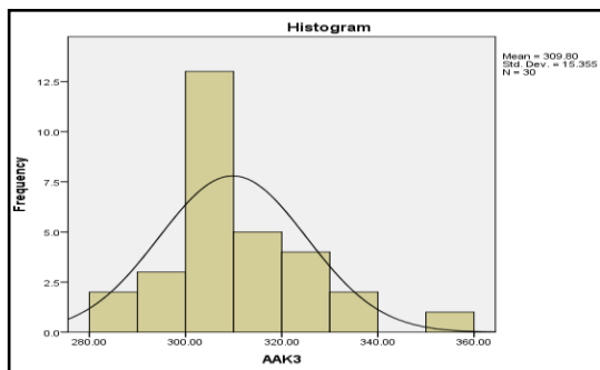
Gambar 4.2 Grafik Histogram AAK 3%
