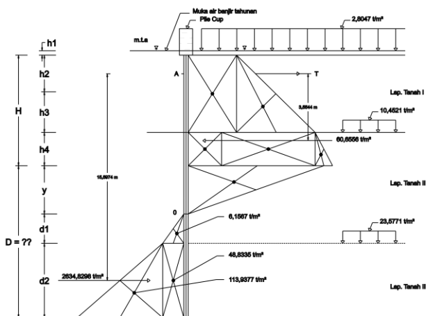
Gambar 4.4 Diagram tekanan tanah pasif
